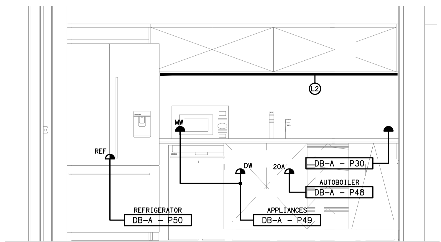
DETAIL A LUNCHROOM KITCHENETTE ELEVATION SCALE 1:20
